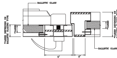
DOOR JAMB AT LOCK
