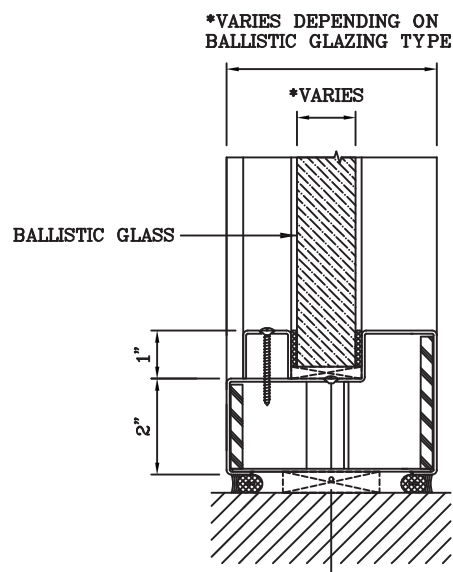
5 SILL DETAIL
