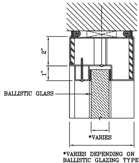
4 HEAD DETAIL
