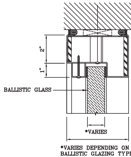
4 HEAD DETAIL
