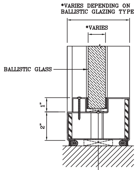
5 SILL DETAIL
