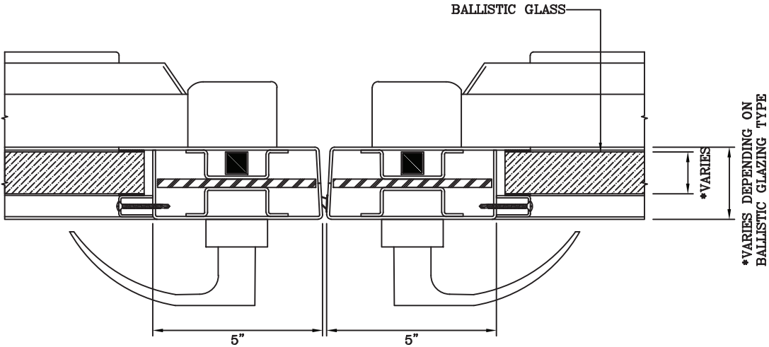
2 - DOOR MEETING STILES DETAIL
