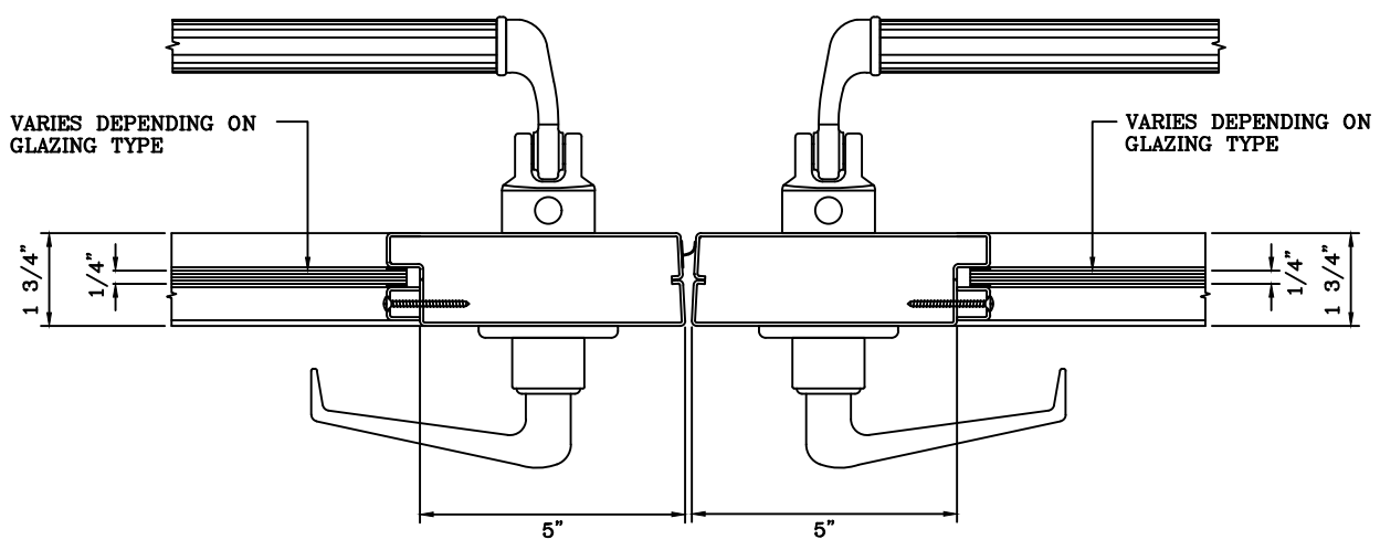
4 DOOR MEETING STILES DETAIL
