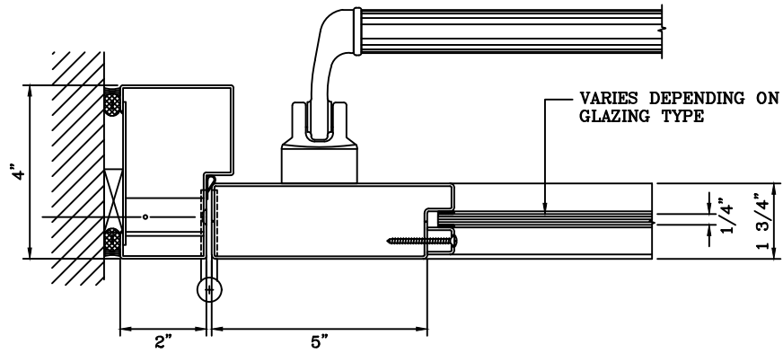
3 DOOR JAMB at HINGE DETAIL
